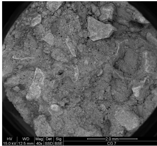
Fig. 1. HA consists of particles of different sizes and shapes incorporated within the biphasic calcium sulfate matrix (scanning electron microscopy).
