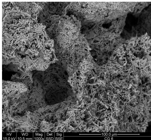
Fig. 2. Postsetting structure of biphasic calcium sulfate at higher magnification, which is composed of needle-like crystals presenting microporosity (1–50 \mu\text{m} ) and macroporosity (300–800 \mu\text{m} ) promoting growth factor infiltration angiogenesis formation and cell proliferation (scanning electron microscopy).
